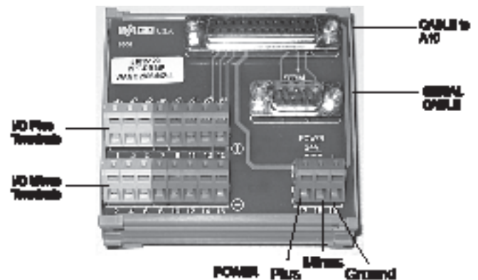
A10 Terminal Block (PPT Part # 248-0138)
